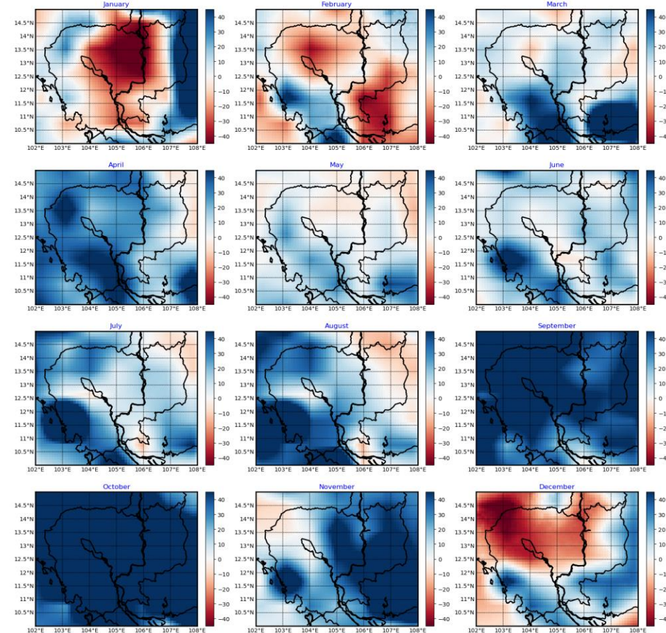
MPI-ESM1-2-HR_ssp585-Climate Change Signal for Far Future(2070-2100)
