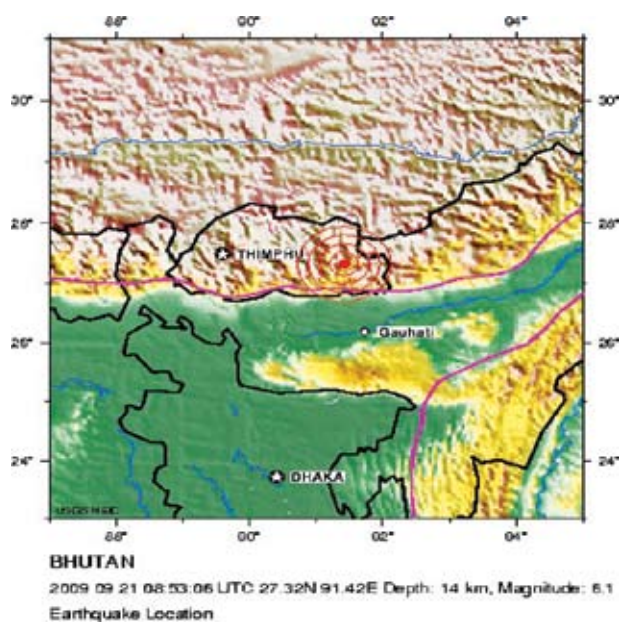
Fig. 1 Earthquake intensity
